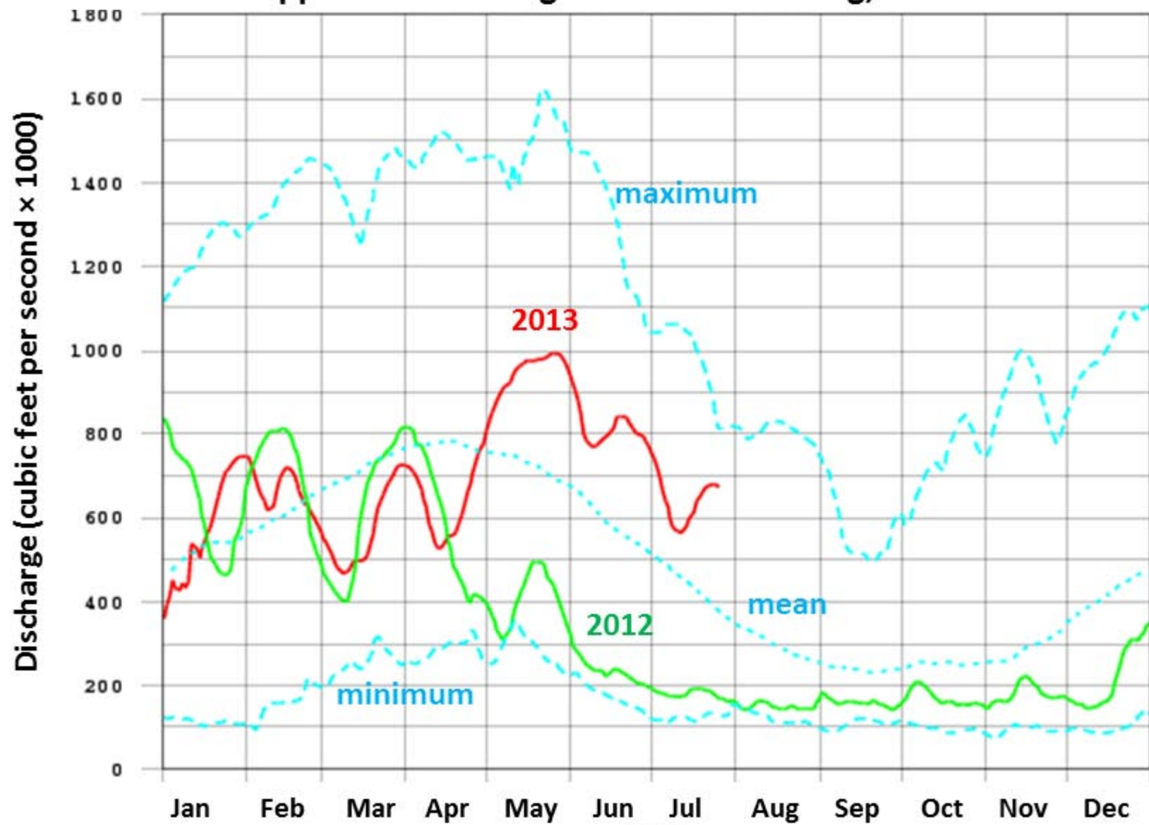
Mississippi River Discharge at Tarbert Landing, 1935-2013
